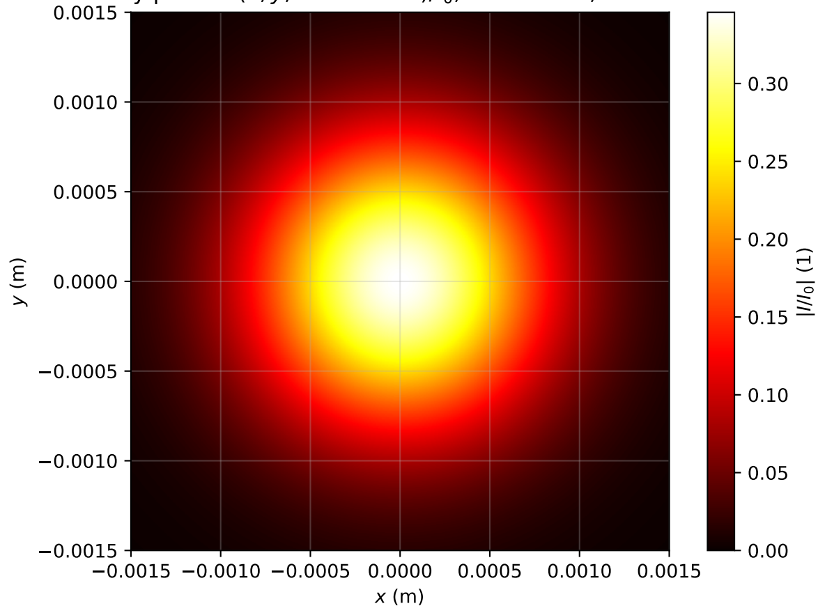
Intensity profile I(x, y, z = 3.184m)/I_0 , P_{in}=0.2P_{cr} , artificial time
